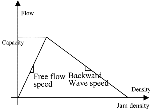
Fig. 1. Assumed two-wave speed flow-density relationship.
